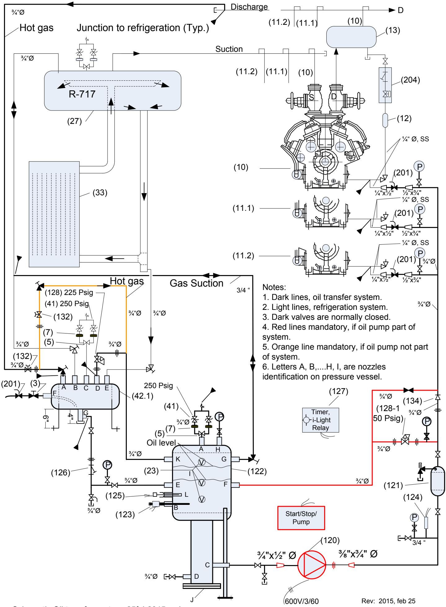
Schematic Oil transfer system_25feb2015.vsd
